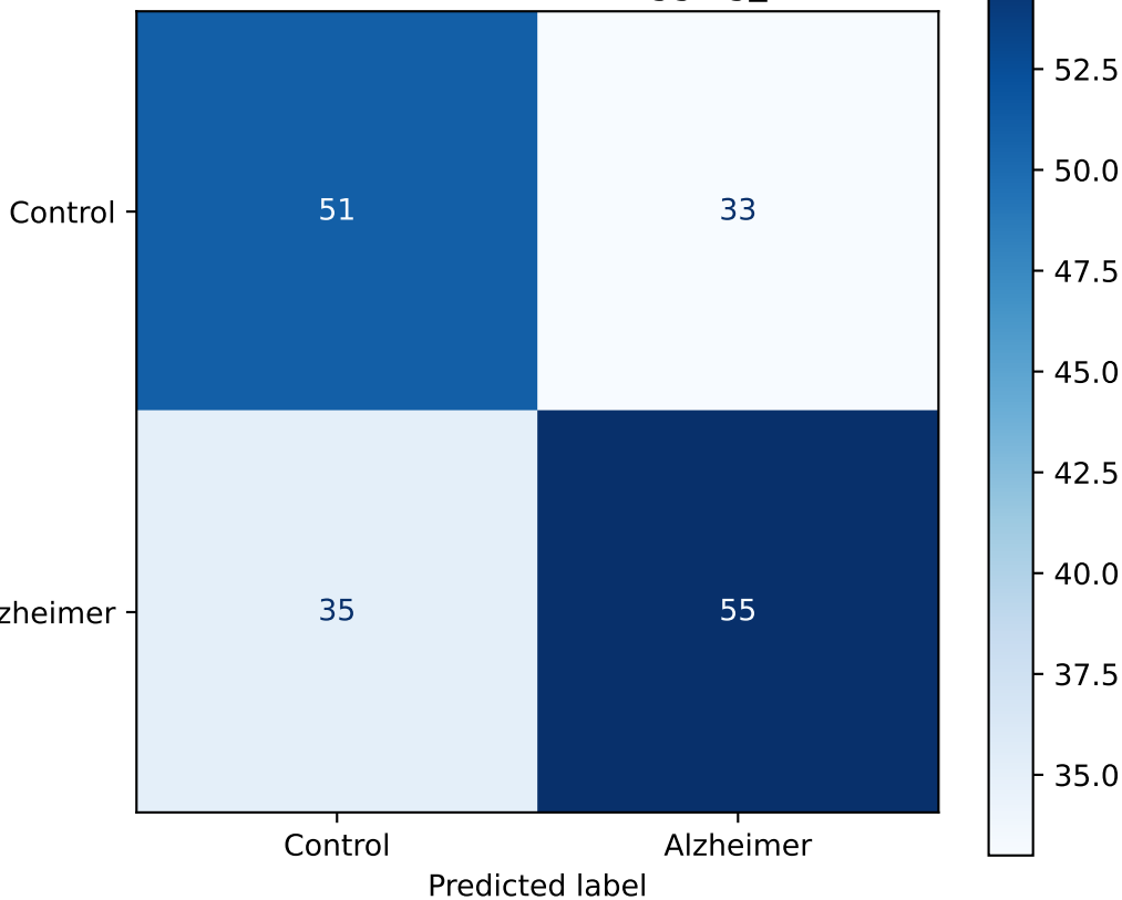
Confusion Matrix - Bagging_LR
